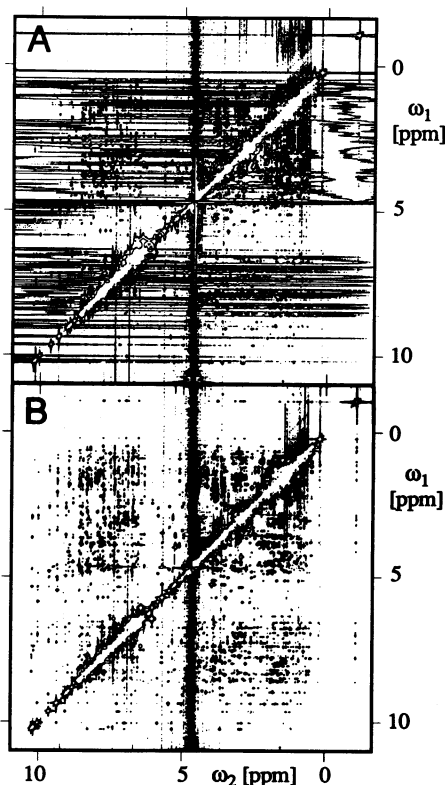
FIG. 1. Contour plots of a NOESY spectrum of Dendrotoxin K (15 mM solution of the protein in 95% H 2 O/5% D 2 O, pH 4.6; temperature, 36°C; proton frequency, 600 MHz; mixing time, 40 ms; recorded time-domain data set with 920 and 2048 data points in the t_1 and t_2 dimensions, respectively; in t_1 the set was zero-filled to 1024 points; cosine filtering in both dimensions; spectral width, 12.62 ppm in both dimensions). Two positive and two negative levels are plotted without distinction; the second contour level is five times higher than the first. (A) Not baseline corrected. (B) Baseline corrected in both dimensions using the program FLATT.
