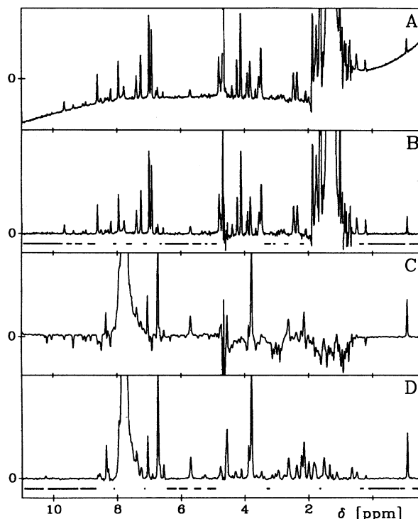
FIG. 2. Cross sections from the NOESY spectra of Fig. 1. In all cases the full spectral width of 12.62 ppm is shown. (A) Row at \omega_1 = 1.34 ppm before baseline correction. (B) Same row as in A after baseline correction in both dimensions. (C) Column at \omega_2 = 7.76 ppm before baseline correction. There are only small baseline distortions in the column, but large artifacts are caused by baseline distortions of the rows, in particular in the region \omega_1 = 0.5 – 3.5 ppm. (D) Same column as in C after baseline correction in both dimensions. The improvement over C is primarily due to the baseline correction of the rows perpendicular to this column. In B and D the pure-baseline regions identified by the program FLATT are indicated by horizontal lines below the spectrum.
