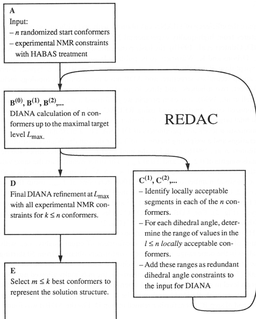
Fig. 1. Flowchart outlining the course of a protein structure calculation with the program DIANA using either the 'direct' way (A-B (0) -D-E) or REDAC (A-B (0) -[C (1) -B (1) ...]-D-E). Typically, the number of REDAC-cycles is 1 or 2.
