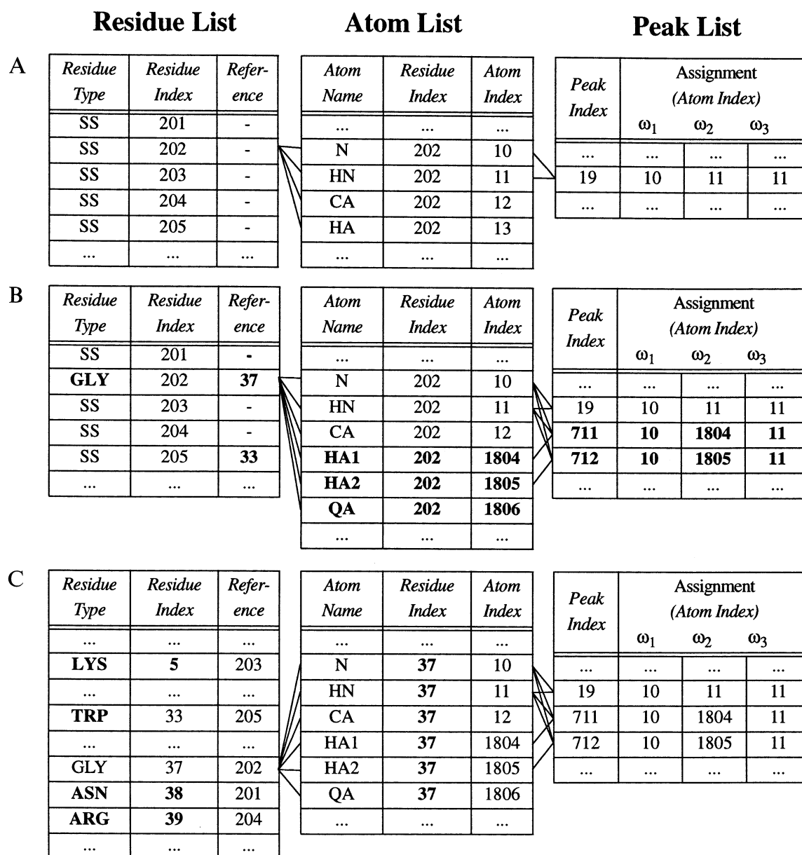
Fig. 2. Data structure used by XEASY for bookkeeping of resonance assignments. A residue list, an atom list and a peak list are used. Lines between the three lists connect entries related by the Residue Index and the Atom Index , respectively. (A) Situation at the outset of the resonance assignment; SS is a generic amino acid residue with atom names attributed only to the backbone fragment that is common to all residues. The assignment given here corresponds to that obtained by picking the diagonal peaks in a 3D ^{15}\text{N} -resolved ^1\text{H} , ^1\text{H} -NOESY spectrum. (B) Situation during the resonance assignment procedure, reflecting the finding that residue 202 corresponds to Gly 37 in the protein sequence, and that the complete Gly 37 spin system has been identified. In the column Atom Name , QA defines a pseudoatom (Wüthrich et al., 1983). Furthermore, without displaying the supporting entries in the atom list and the peak list, the residue list indicates that residue 205 is in position 33 in the protein sequence. The temporary sequence numbers of the residues are listed in the Reference column. (C) Situation after completion of the resonance assignments: the Residue Type and Residue Index entries now refer to the amino acid sequence of the protein, where the supporting entries in the atom list and the peak list are given only for Gly 37 ; the original Residue Index is kept in the column Reference . Bold entries in (B) and (C) emphasize changes in the lists compared to situations (A) and (B), respectively. See text for further details on the use of this data structure.
