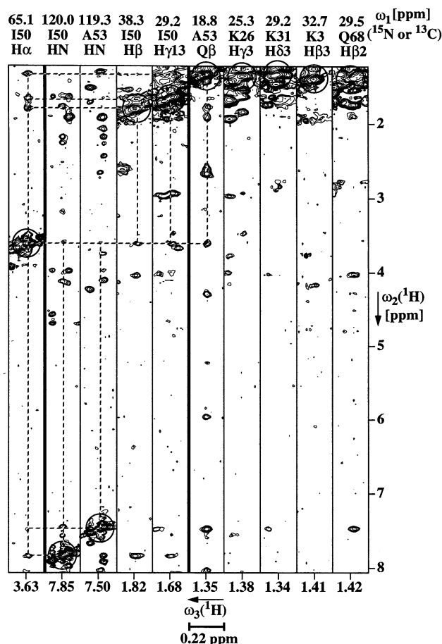
Fig. 6. Illustration of cross-peak assignments in 3D heteronuclear-resolved ^1\text{H} , ^1\text{H} -NOESY spectra (Fesik and Zuiderweg, 1988; Ikura et al., 1989). The example is from the ^{15}\text{N} , ^{13}\text{C} doubly labeled N-terminal domain of the protein DnaJ (Szyperski et al, 1994b). Strips for individual protons are defined as in Fig. 5, where the strips 1 and 4–10 are from the ^{13}\text{C} -resolved ^1\text{H} , ^1\text{H} -NOESY spectrum, and strips 2 and 3 from ^{15}\text{N} -resolved ^1\text{H} , ^1\text{H} -NOESY. Diagonal peaks are encircled. The snapshot was taken after the assignment of the cross peaks between Ile 50 H \alpha and Ile 50 H \gamma , Ala 53 H \gamma , Ile 50 H \beta and Ile 50 H \gamma was completed, and assignment of the cross peak at 1.35 ppm in the strip of Ile 50 H \alpha was in progress. Cross peaks involving Ile 50 H \alpha are connected to the corresponding diagonal peaks in the other strips by broken lines, i.e., the protons corresponding to the ^1\text{H} - ^1\text{H} diagonal peaks in strips 2–5 define the assignment of the coupled hydrogen atom manifested in the cross peak in the strip of Ile 50 . Strips 6–10 are candidates provided by XEASY for the assignment of the cross peak at 1.35 ppm. They are sorted by increasing distance of their diagonal peak (encircled) to this cross peak and the similarity of their peak patterns with the pattern observed in strip 1 (Eq. 1). Since only the strip of Ala 53 Q \beta lies exactly at 1.35 ppm and also shows a cross peak to Ile 50 H \alpha , visual inspection readily confirmed the validity of the automatic strip ranking by XEASY.
