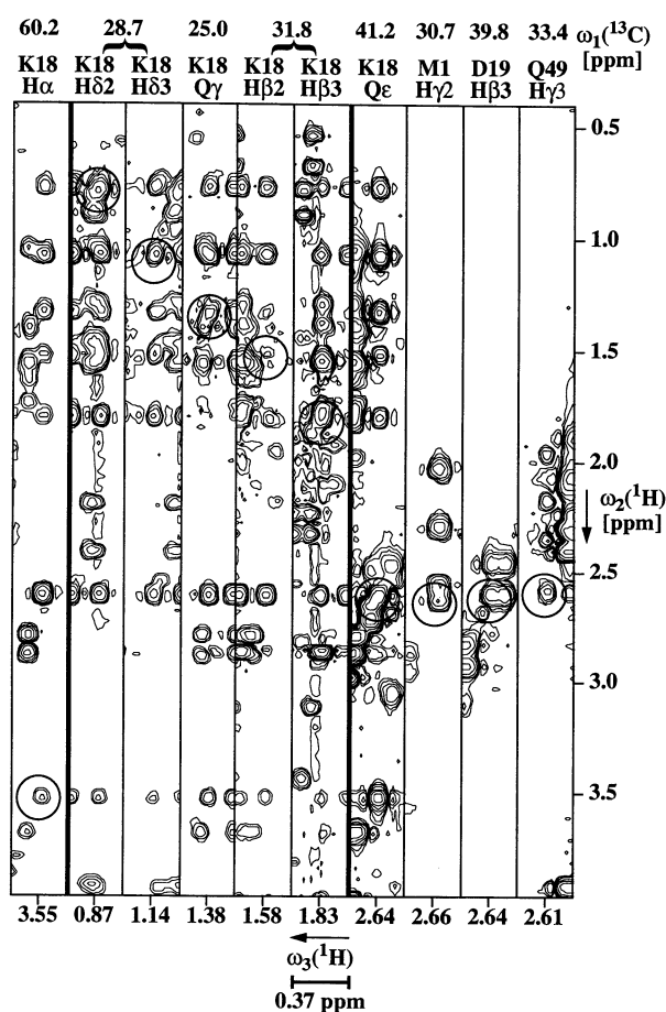
Fig. 5. Spin system identification in an [HCCH]-TOCSY spectrum (Bax et al., 1990) using XEASY, illustrated with the [^{15}N, ^{13}C] -labeled mixed disulfide between E. coli glutaredoxin and glutathione (Bushweller et al., 1994). The assignment above each strip is for the residue and the proton type corresponding to the encircled diagonal peak. In \omega_1 the strips are at the ^{13}C positions of these encircled peaks, and along \omega_3 they are centered about the proton frequency of these peaks. The frequencies of the encircled peaks prior to any folding operation (see also Fig. 3) are listed above and below each strip. From left to right we refer to the strips as 1 to 10. Strip 1 corresponds to H^{\alpha} of Lys 18 and is used as a reference to search for the remaining strips of the Lys 18 spin system. At the stage of the analysis illustrated here, strips 2–6 had already been found to correspond to the same spin system as strip 1. Strips 7–10 are candidates provided by XEASY for the strip of \epsilon CH_2 , based on the small distance between the diagonal peaks (encircled) and the remaining cross peak in strip 1, and the similarity of their peak patterns with the pattern observed in strip 1 (Eq. 1). From the complete peak pattern, the strip at ( \omega_1=41.2 ppm, \omega_3=2.64 ppm) could then be identified as belonging to the same spin system as the reference strip, either from the value of the dot-product correlation function (Eq. 1), or interactively by visual inspection.
